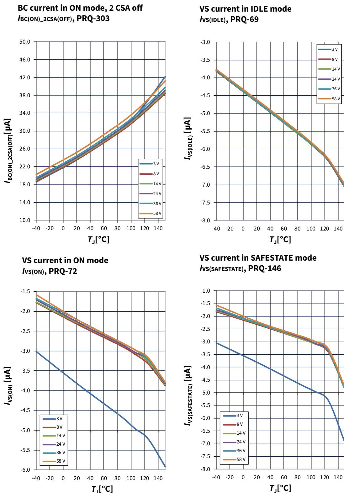
Figure 30 Current consumption continued
