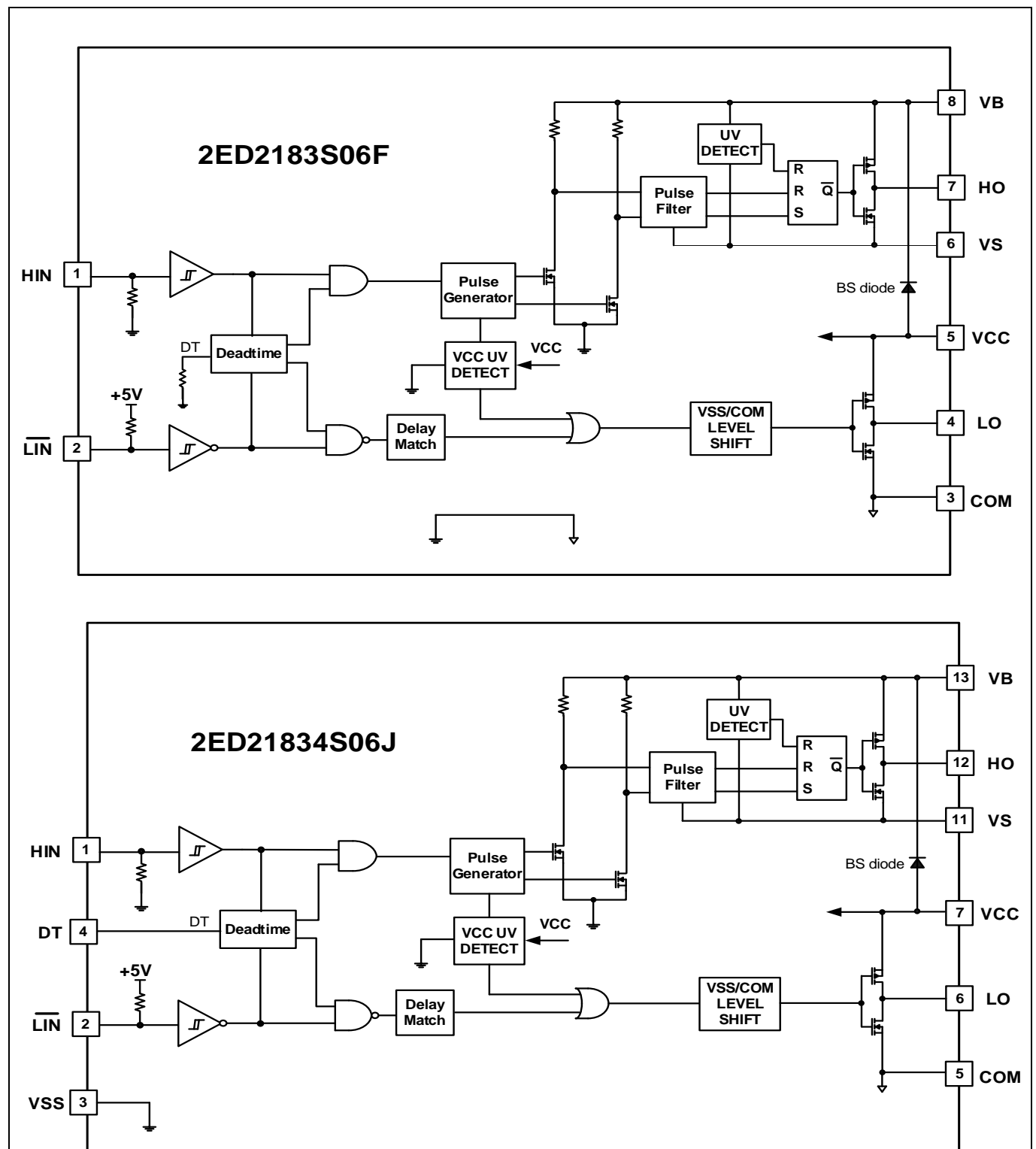
Figure 2 Block diagrams
