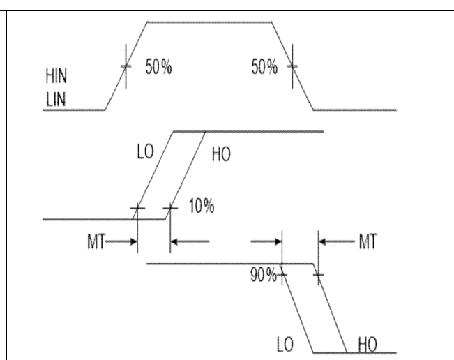
Figure 9 Delay Matching Waveform Definitions
