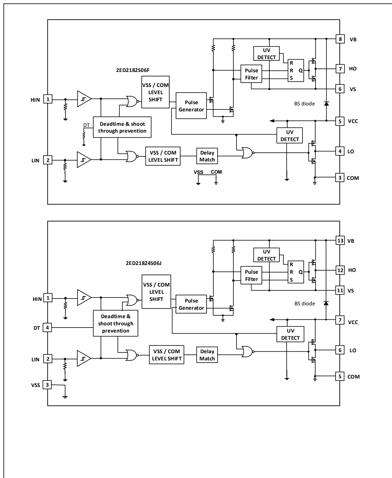
Figure 2 Block diagrams
