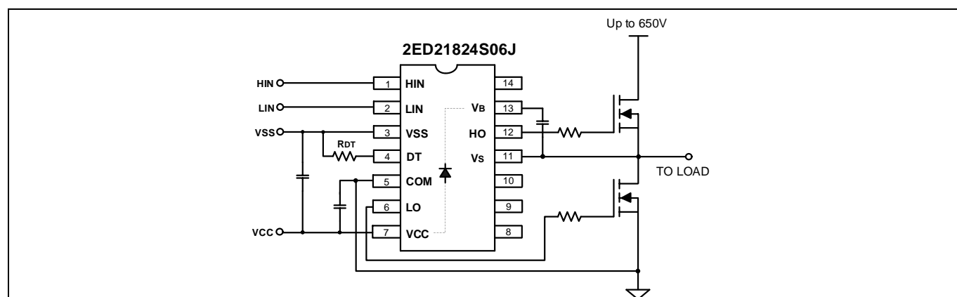
Figure 10 14-pin half-bridge variants having adjustable dead-time feature settable with a resistor
