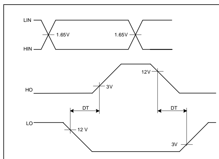
Figure 8 Dead Time Definitions
