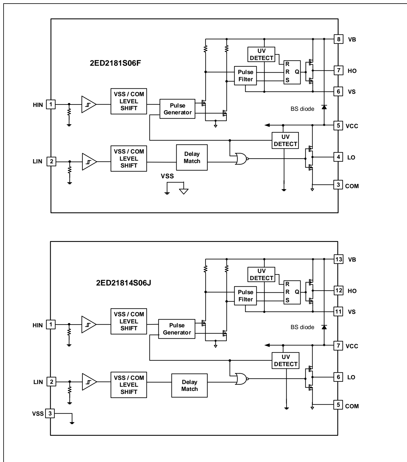
Figure 2 Block diagrams
