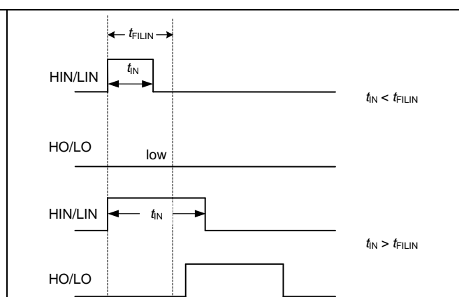
Figure 7 Input filter
