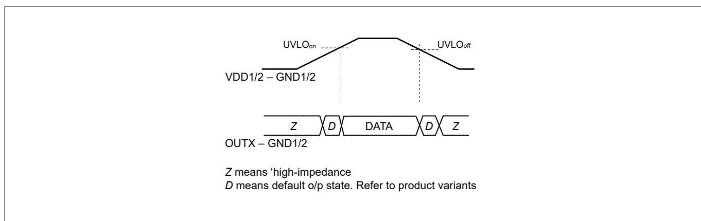
Figure 8 Under-voltage lockout
