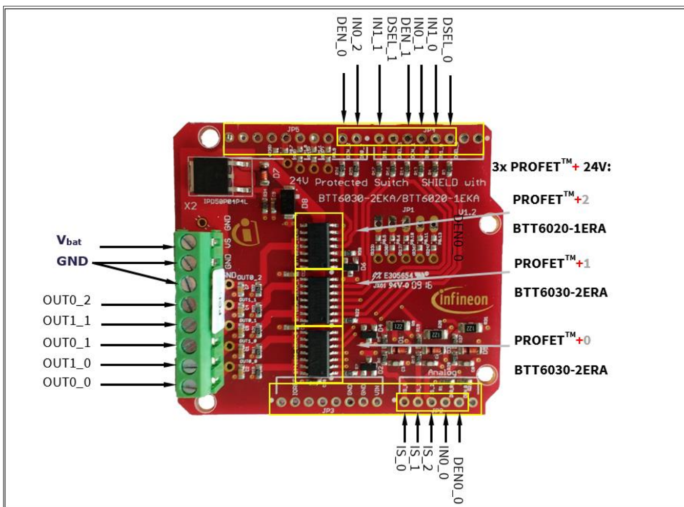
Figure 1 24V Protected Switch Shield photo
