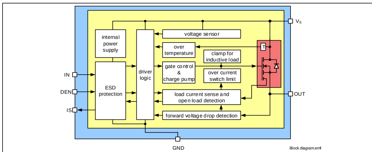
Figure 13 Block diagram BTT6020-1ERA
