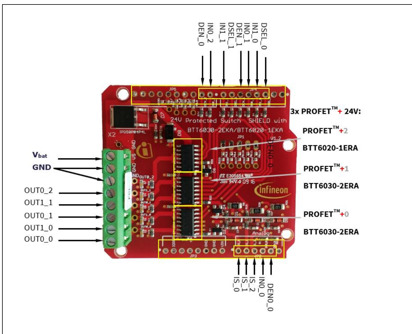
Figure 8 24V Protected Switch Shield connectors
