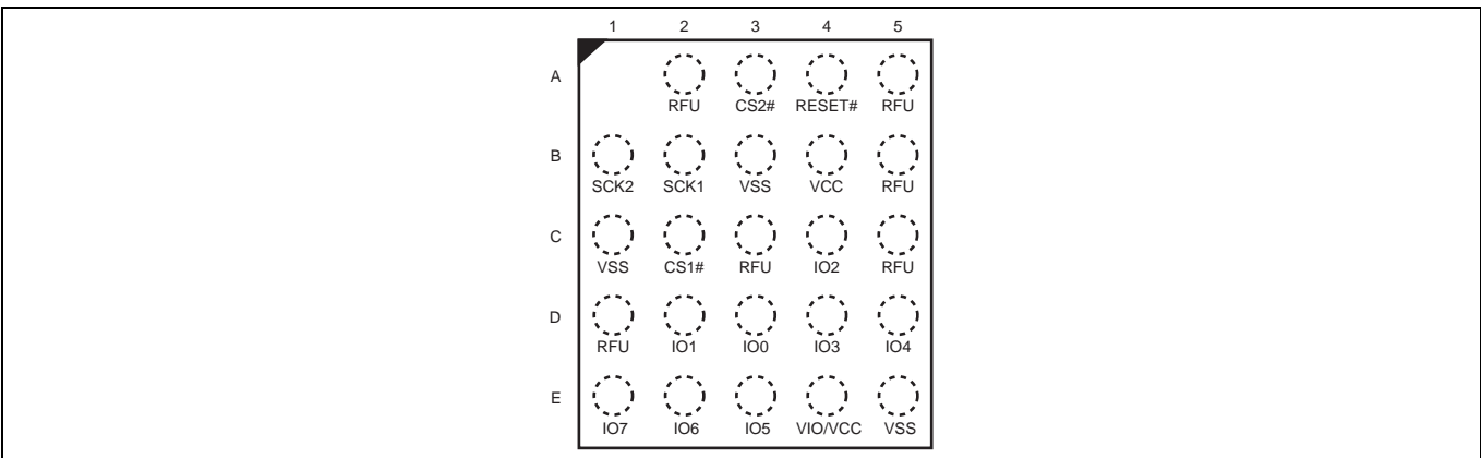
Figure 27 Dual-Quad 24-ball BGA, 5 x 5 ball footprint (ZSA024), top view
