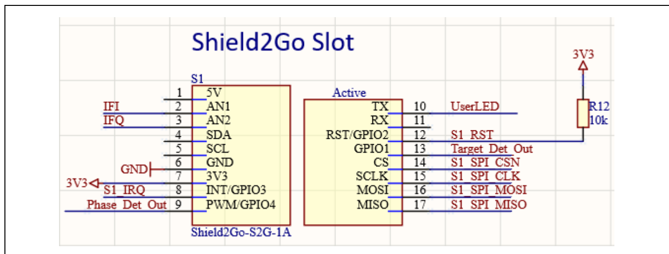
Figure 5 Shield2Go connector S1 schematics
