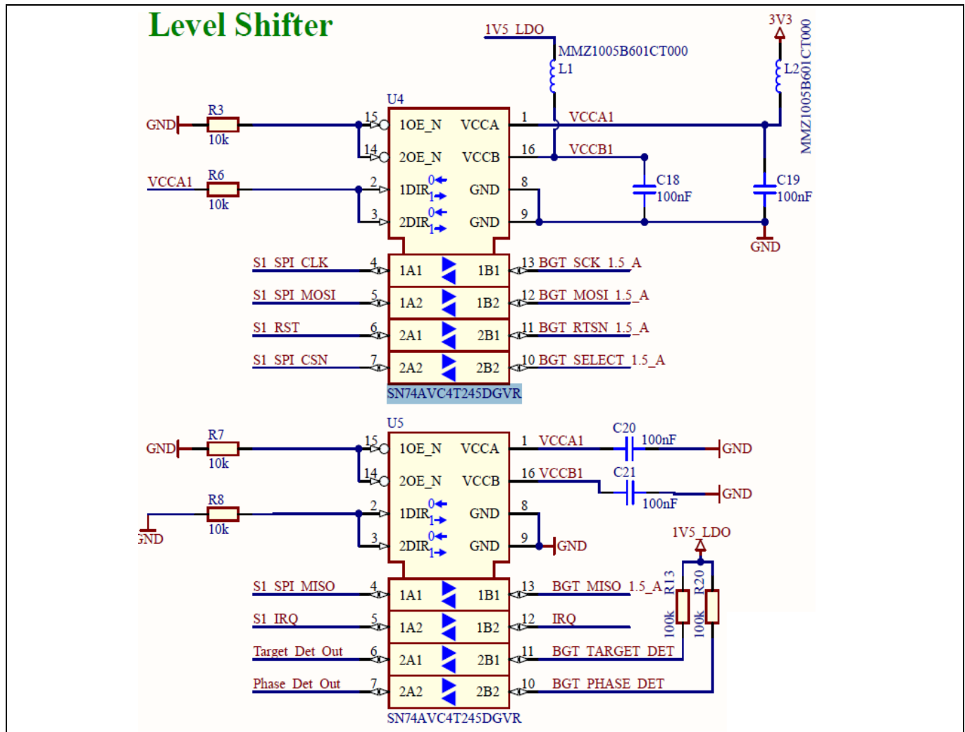
Figure 17 Level shifter circuit (3.3 V to 1.5 V, and vice versa)
