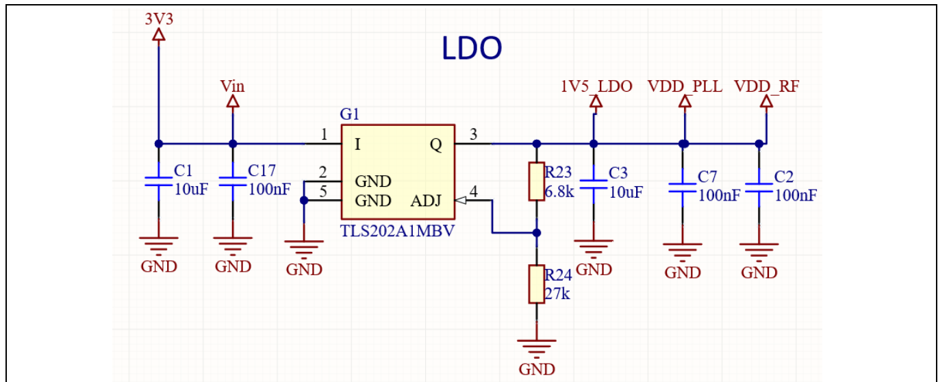
Figure 16 Power supply circuit
