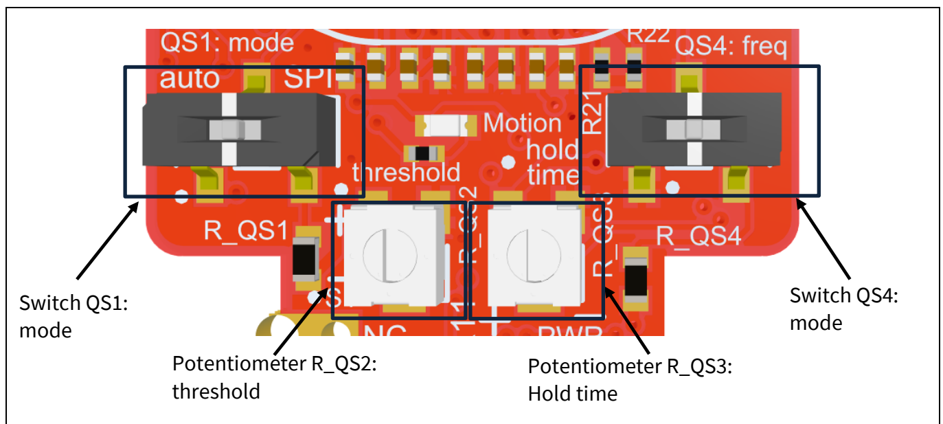
Figure 13 Overview of QS1 to QS4 signals on the BGT60LTR11AIP Radar Shield2Go from the top
