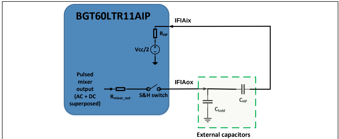
Figure 21 Internal circuit of the BGT60LTR11AIP connected with adjustable external capacitors
