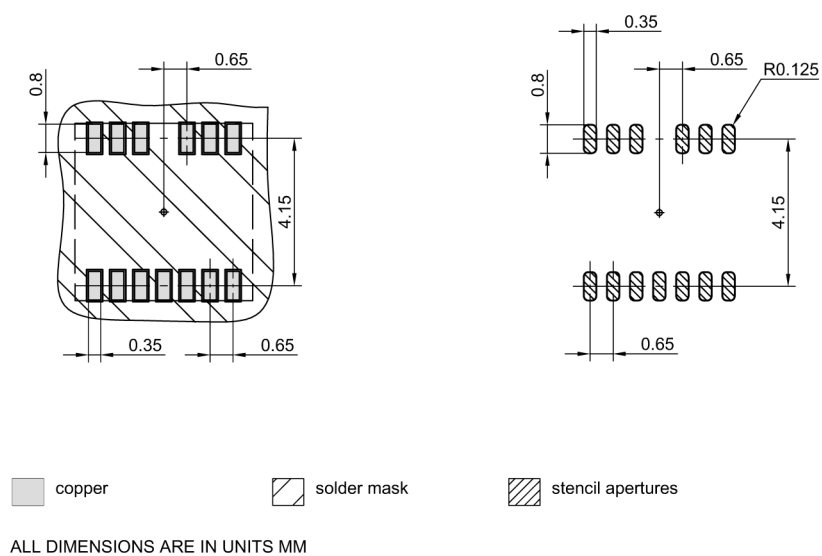
Figure 23 PG-TFLGA-13-1 footprint
