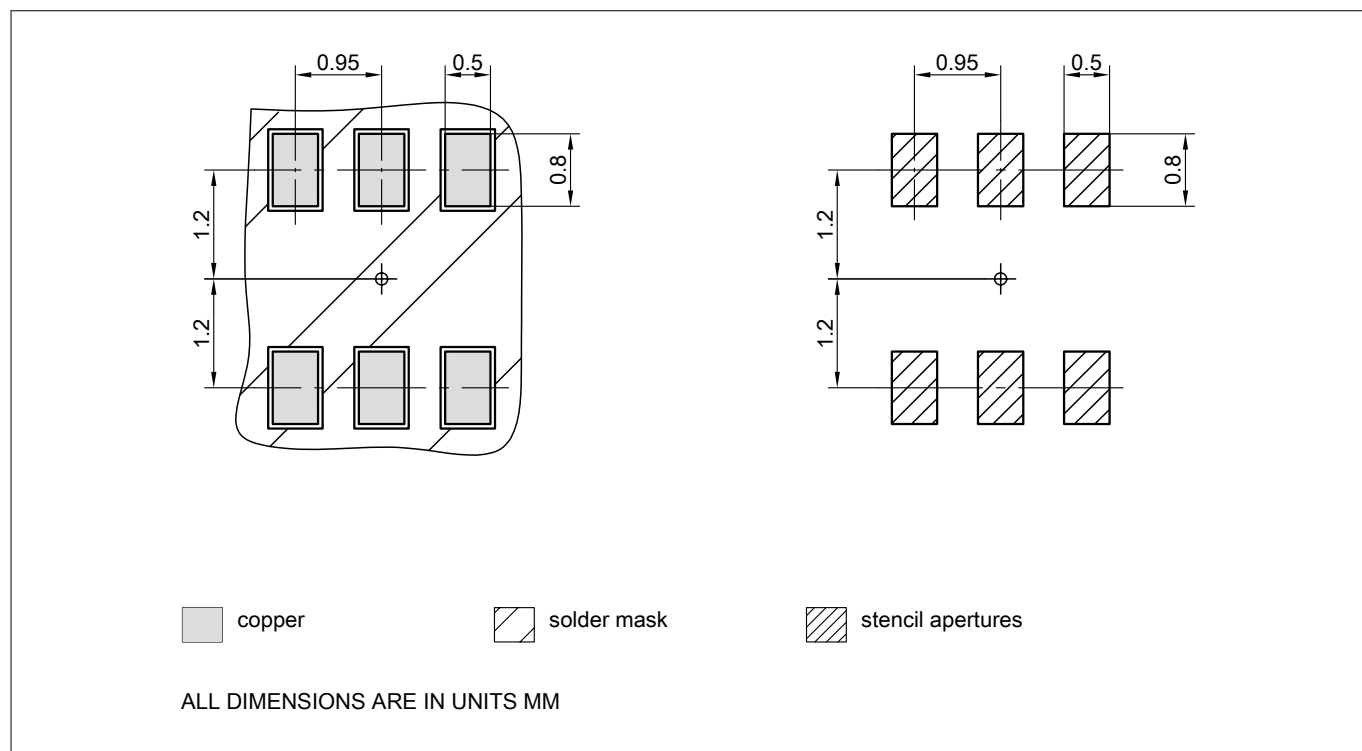
Figure 16 PG-SOT23-6 footprint
