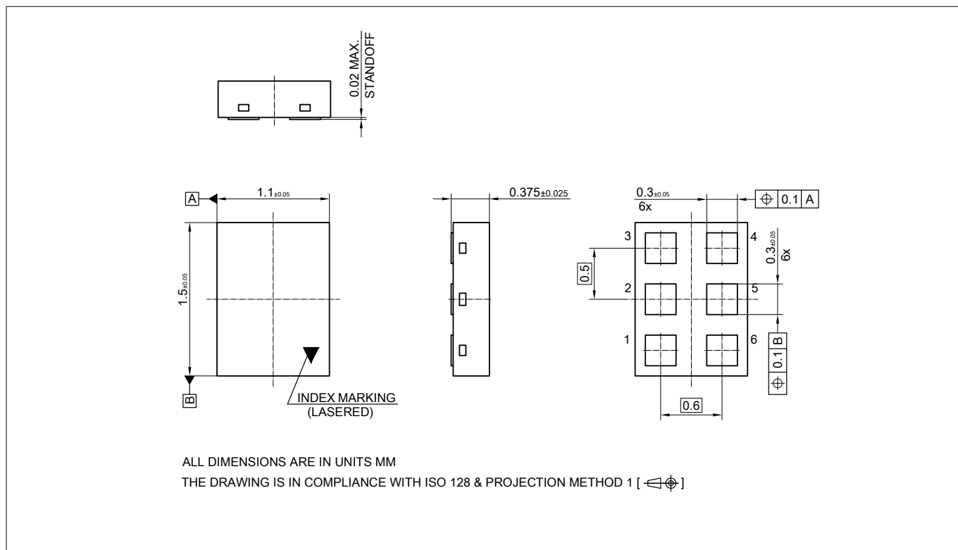
Figure 19 PG-TSNP-6 outline
