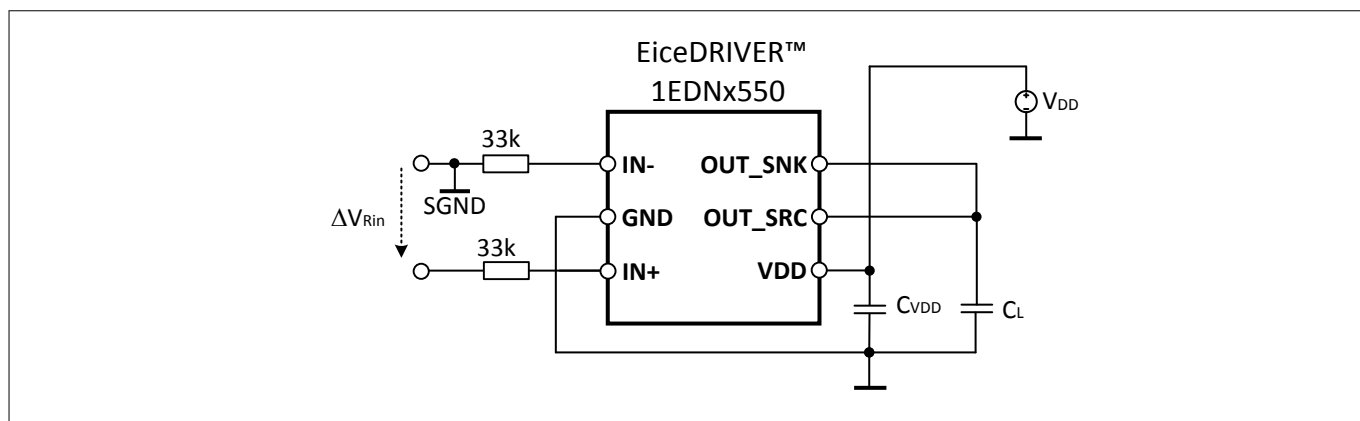
Figure 5 Test circuit
