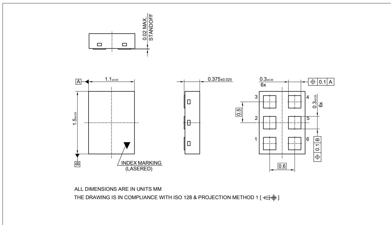
Figure 19 PG-TSNP-6 outline
