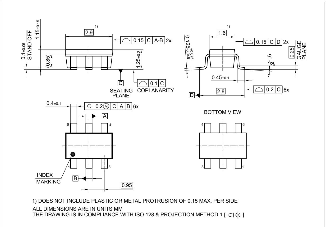
Figure 15 PG-SOT23-6 outline
