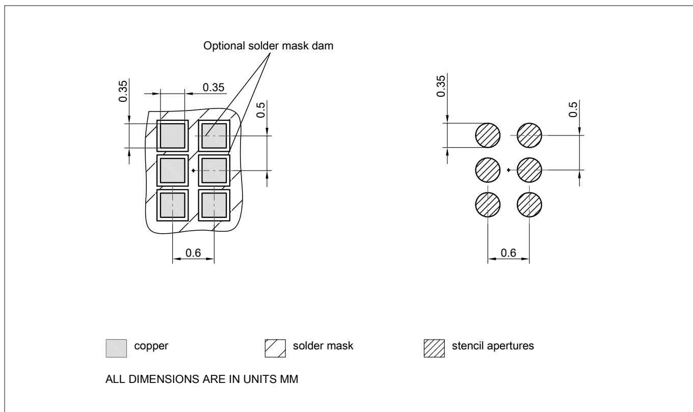
Figure 20 PG-TSNP-6 footprint
