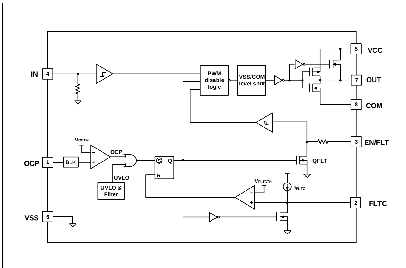
Figure 2 Block diagram
