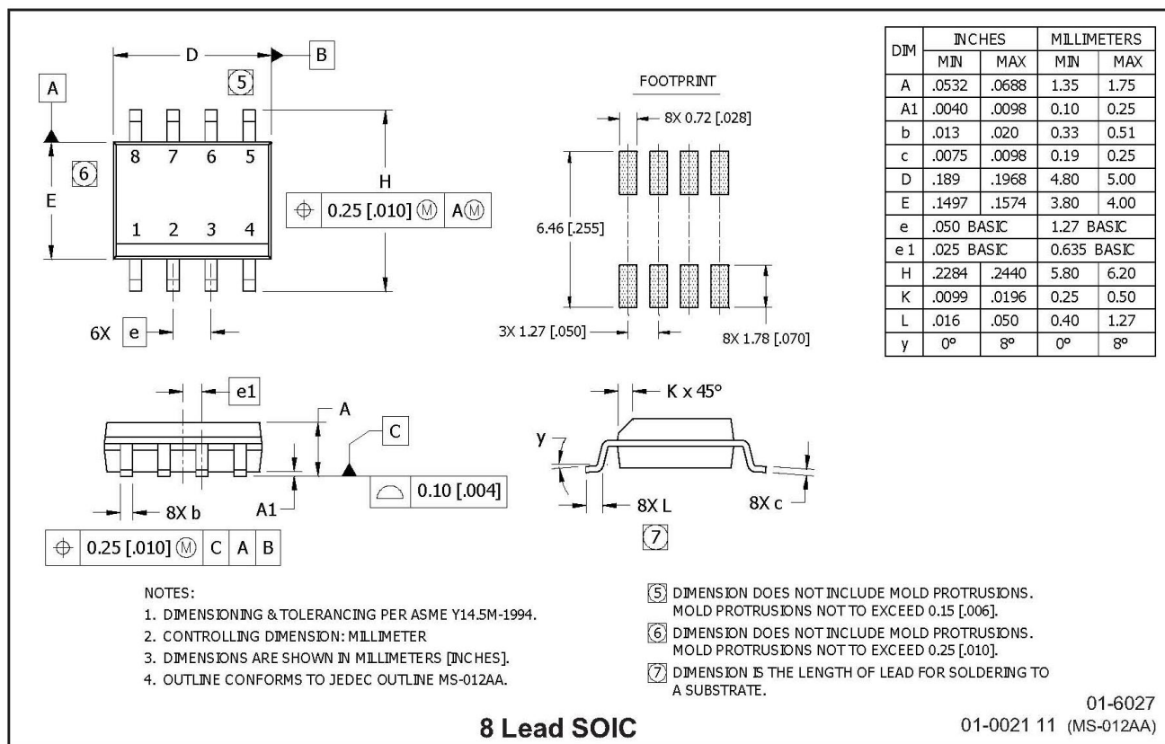
Figure 16 Package outline
