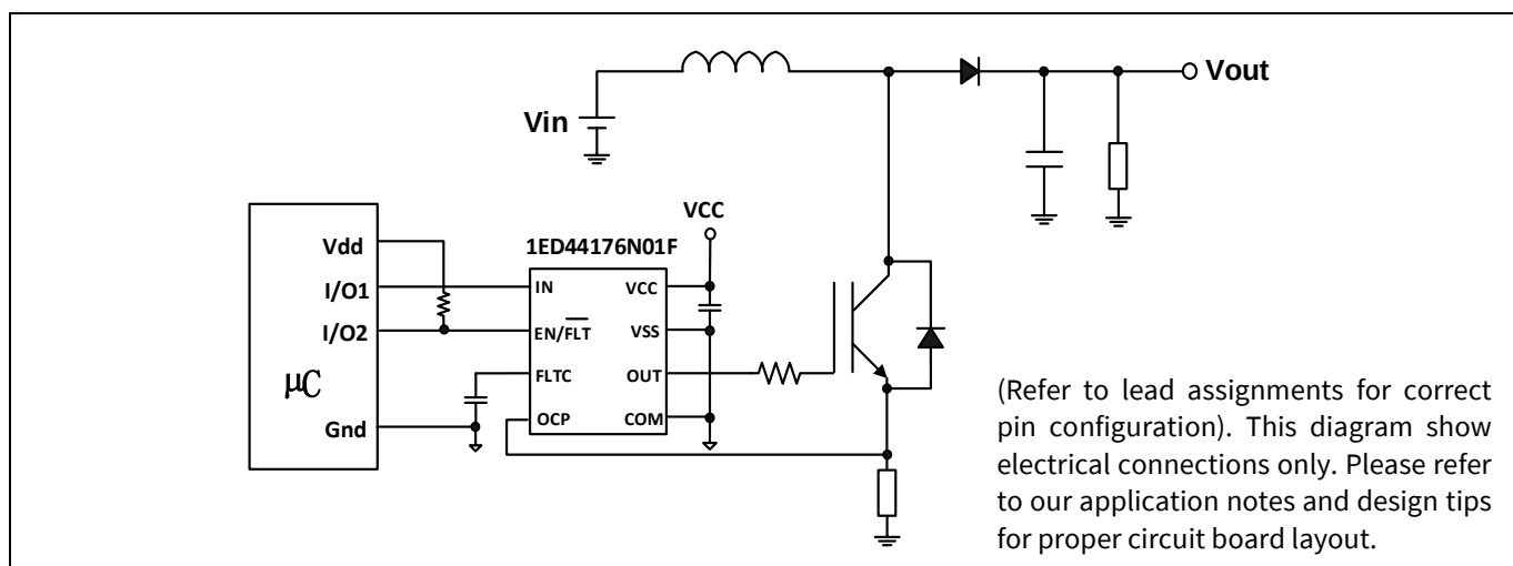
Figure 1 Typical application
