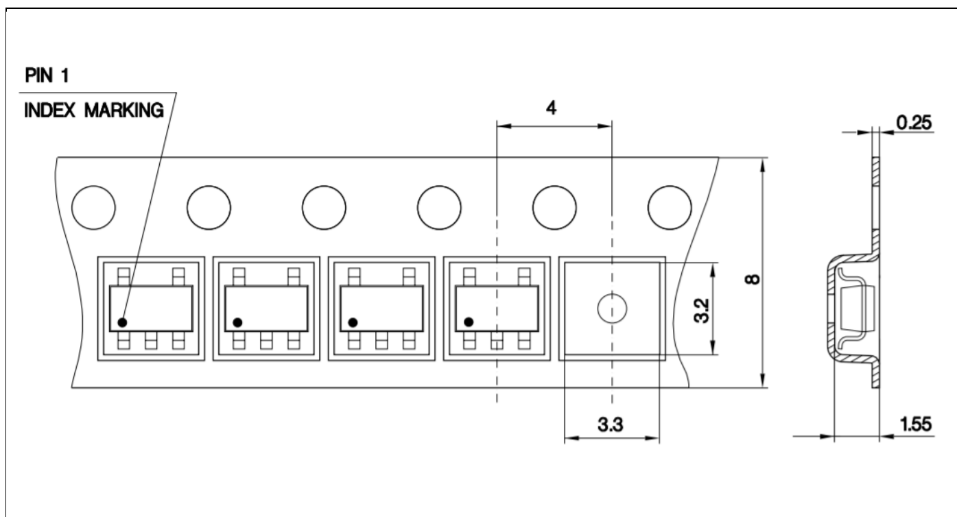
Figure 14 Tape and reel dimensions
