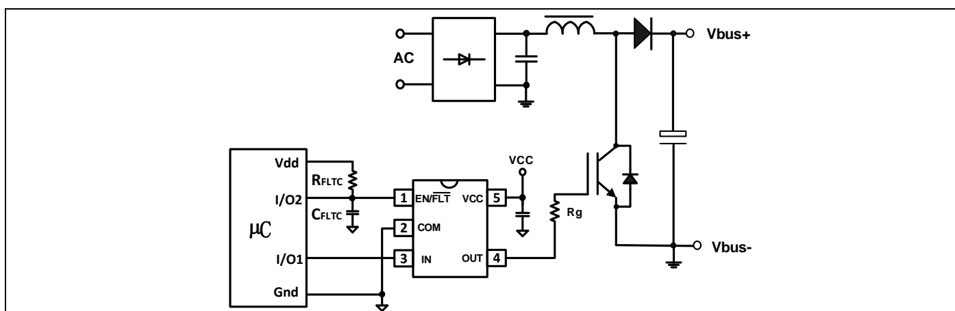
Figure 9 1ED44171N01B in Boost application
