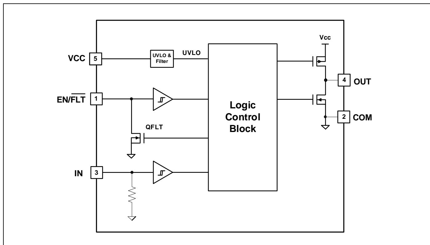
Figure 2 Block diagram
