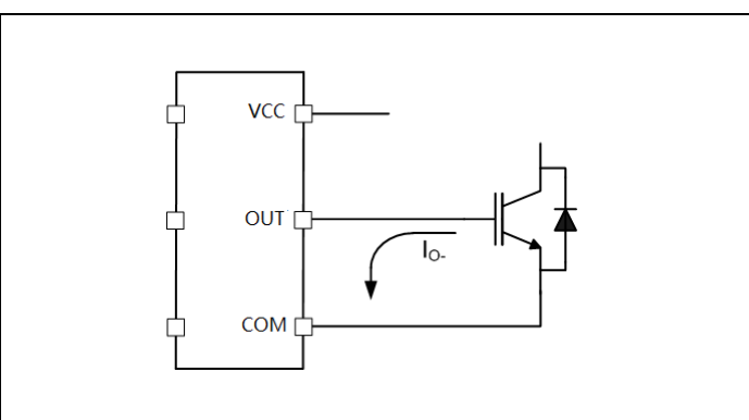
Figure 5 Gate output sinking current
