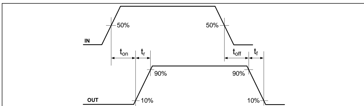
Figure 6 Switching time waveforms
