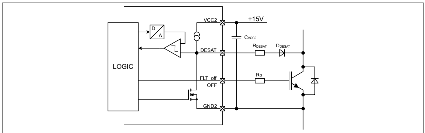
The 1ED34x1Mc12M family (X3 Analog) has a fixed DESAT threshold level of typical 9.18 V. If lower threshold levels are required, the DESAT resistor can be increased. Larger DESAT resistor values lead to lower DESAT threshold voltages. The threshold voltage reduction is equal to the DESAT current multiplied by the DESAT resistance.
