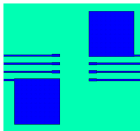
Figure 10 Reference layout for thermal data (Copper thickness 35 μm)
