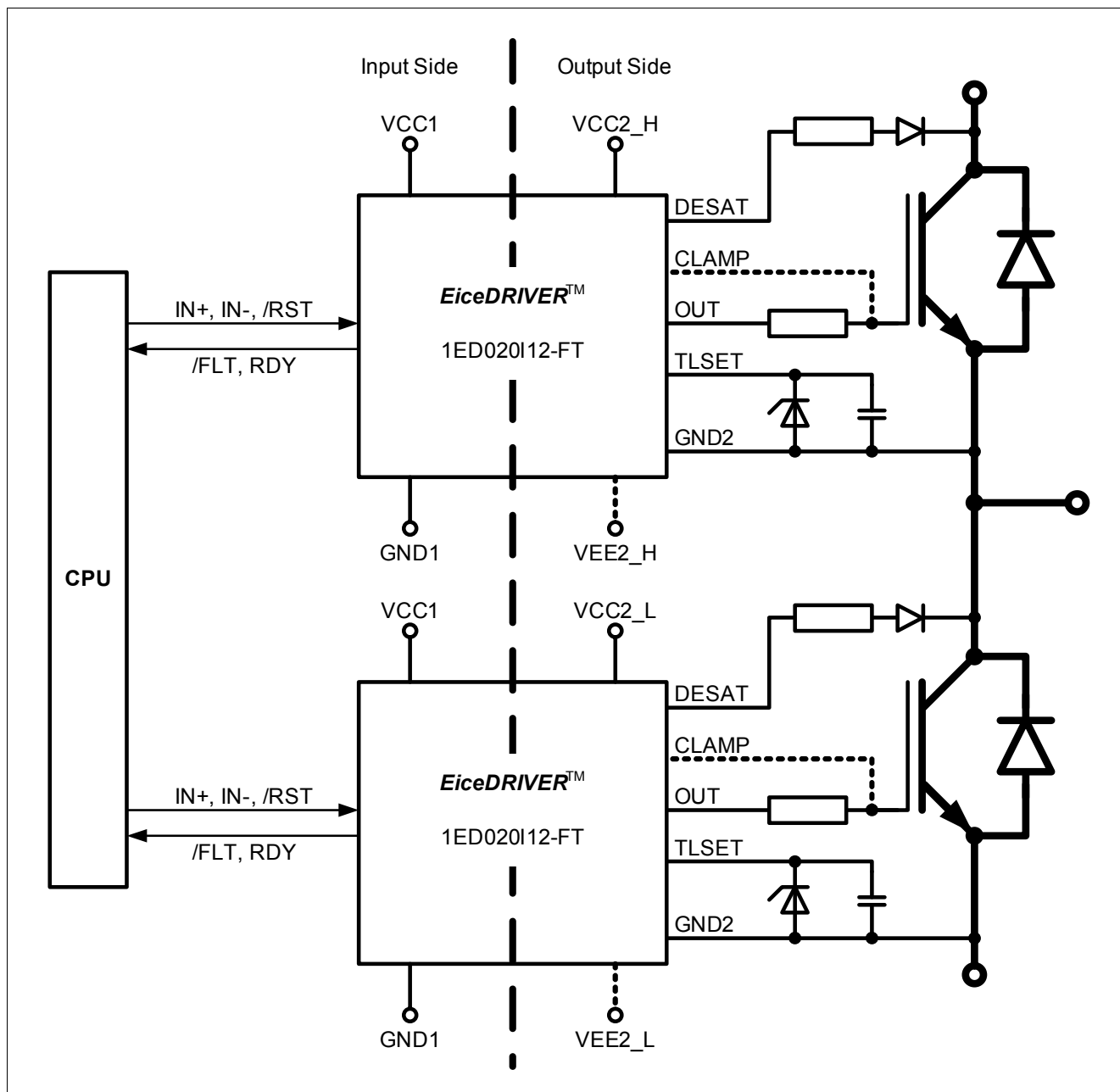
Figure 1 Typical Application
