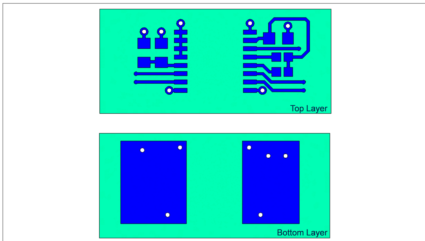
Figure 11 Reference layout for thermal data (Copper thickness 102 \mu m)
