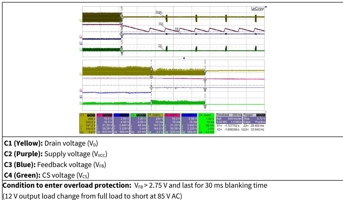
Figure 30 Overload protection
