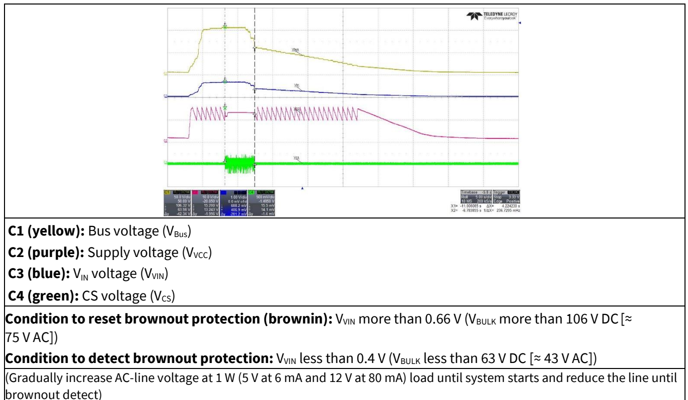
Figure 27 Brownout protection
