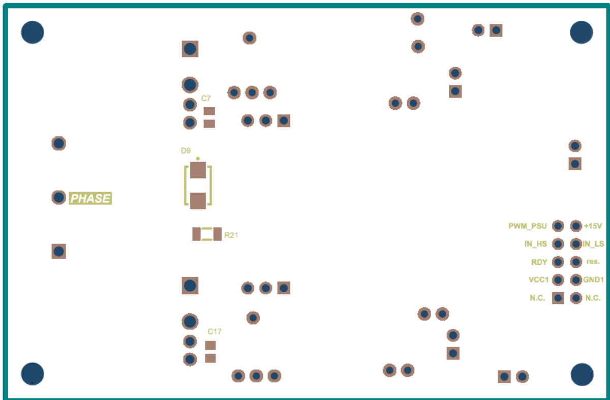
Figure 12 PCB bottom side
