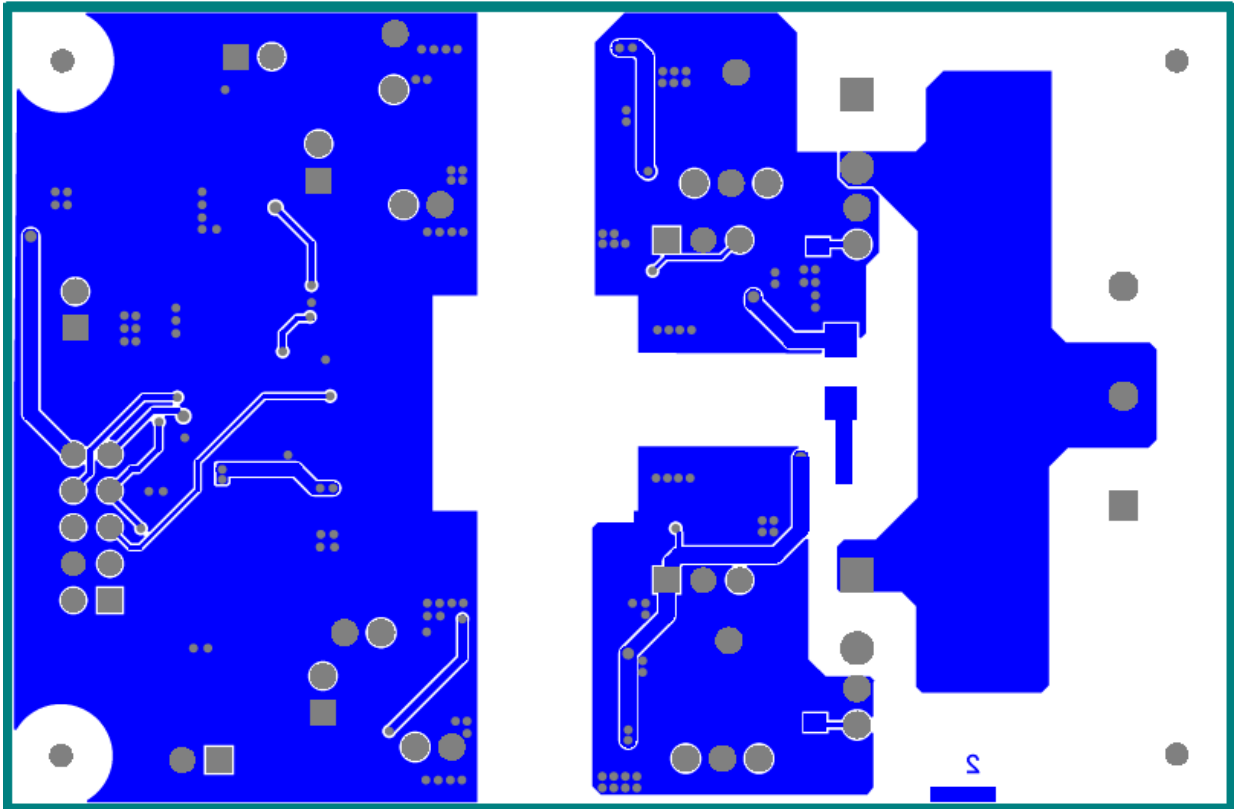
Figure 11 PCB bottom copper layer
