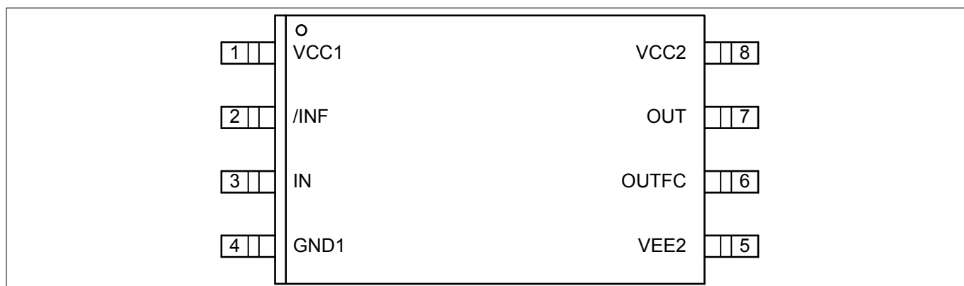
Figure 4 Pinout clamp configuration (top view)
