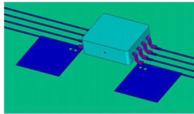
Figure 8 Reference layout for thermal data (1s0p, 2 x 50 mm 2 cooling area, Copper thickness 35 \mu m )
