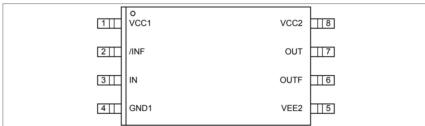
Figure 3 Pinout standard configuration (top view)
