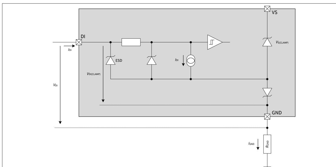
Figure 11 Input circuitry
