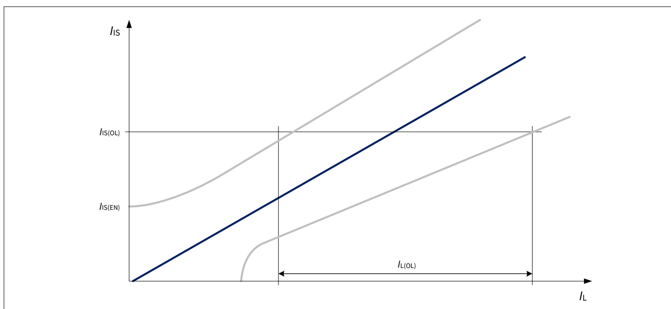
Figure 30 Current sense ratio in open load at ON condition
