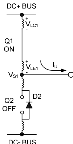
Figure 26: V_S positive
