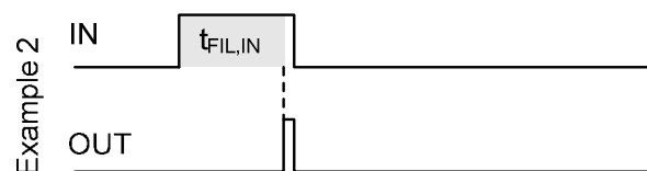
Figure 12: Typical input filter
