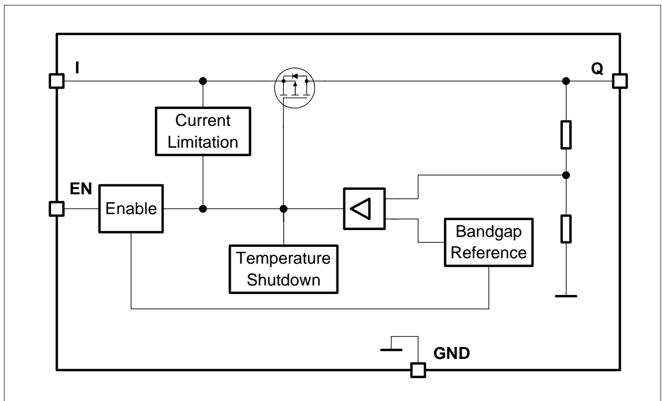
Figure 1 Block Diagram of TLS710/715B0
