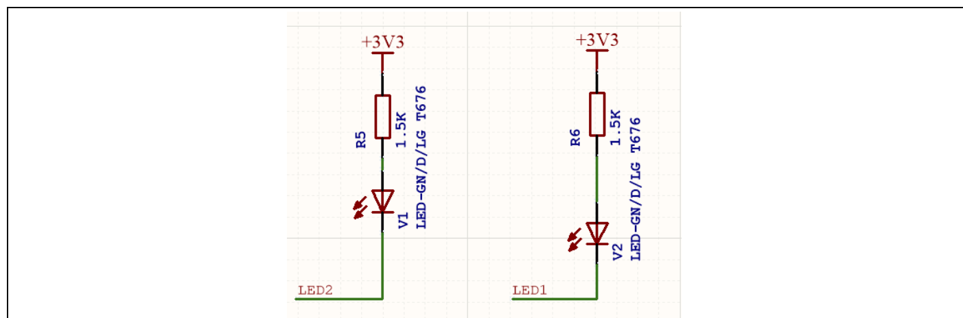
Figure 7 LEDs circuit
