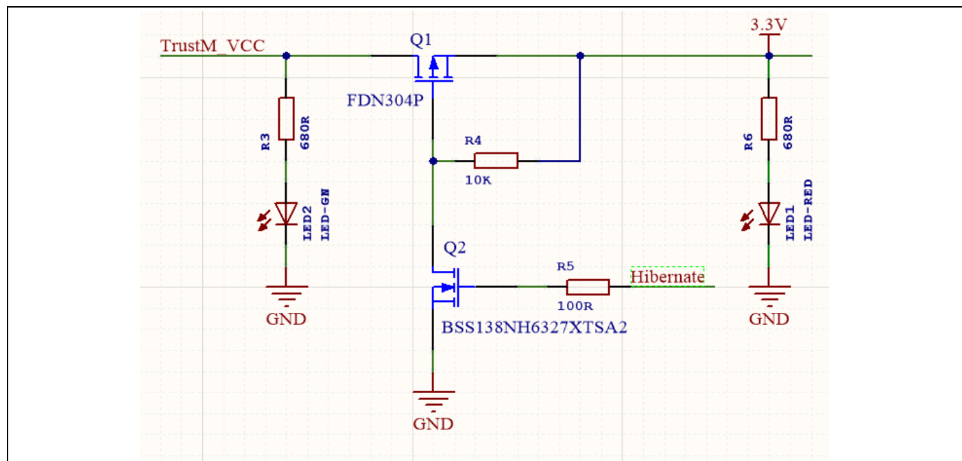
Figure 26 OPTIGA™ Trust M Hibernation reference circuit.
