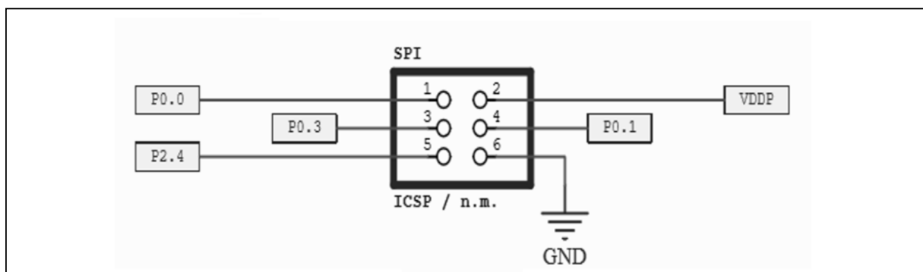
Figure 6 ICSP connector
