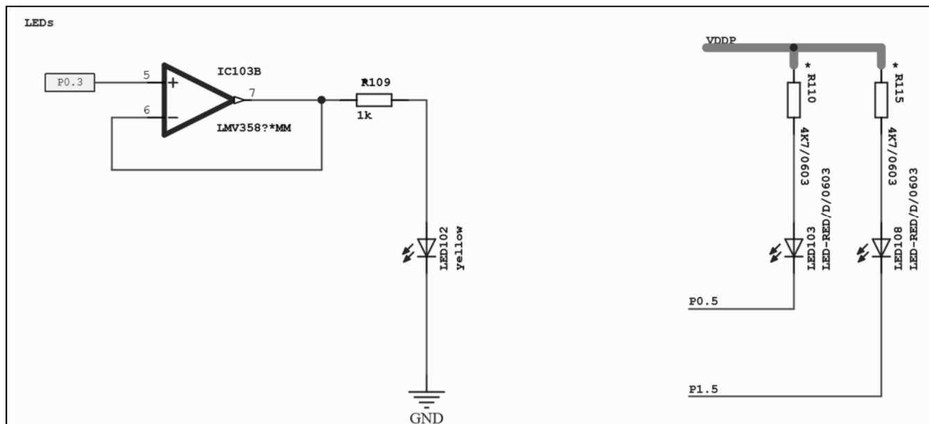
Figure 7 LEDs Circuit
