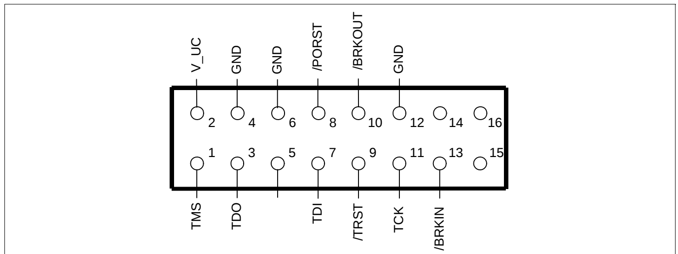
Figure 6-11 OCDS1 connector pinout (IDC16)
