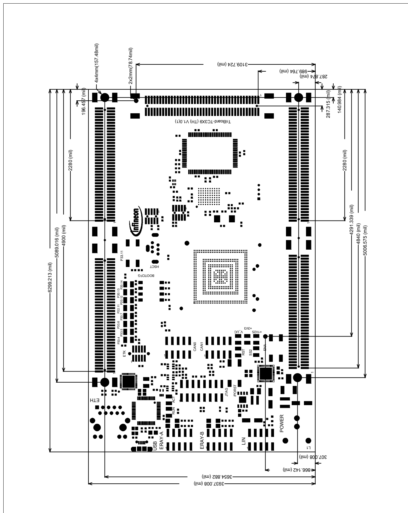
Figure 7-14 Dimensioning (mil)
