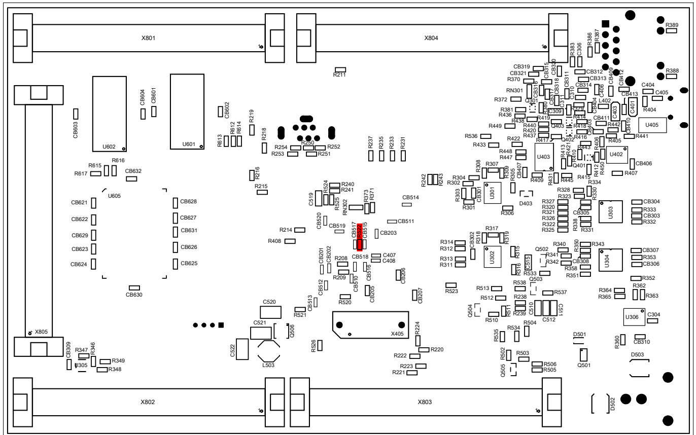
Figure 3-7 Resistor for VDDSB on TriBoard TC3X9 V1.0
