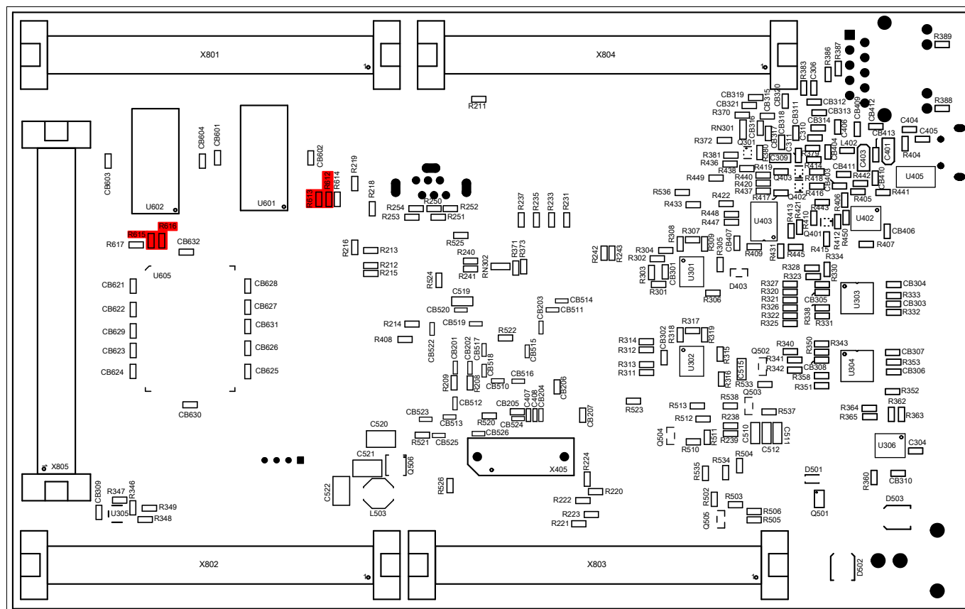
Figure 4-7 Location of memories resistors on Bottom Side
