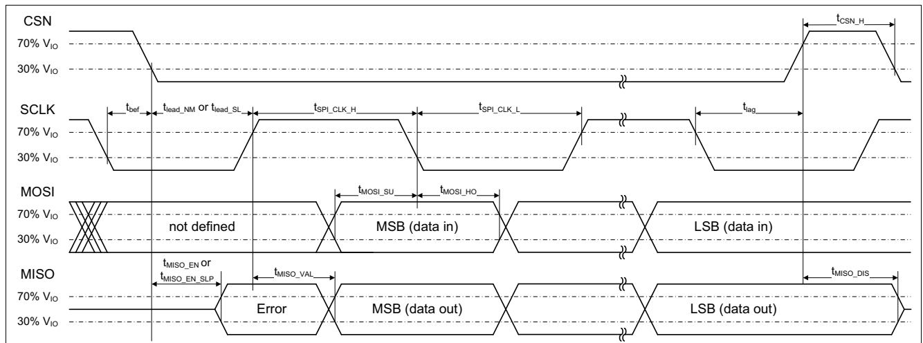
Figure 52 SPI timings
