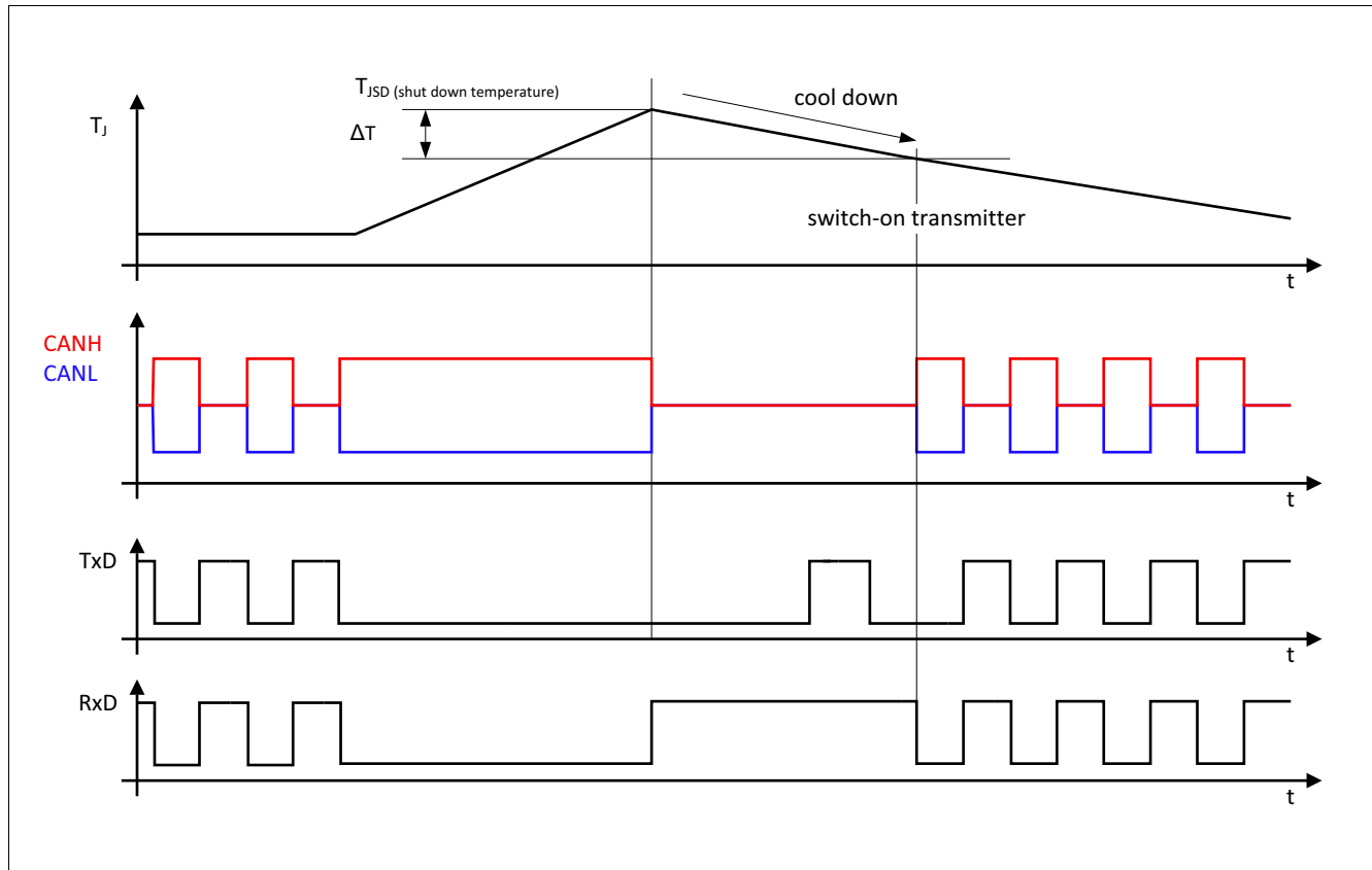
Figure 35 Overtemperature protection
