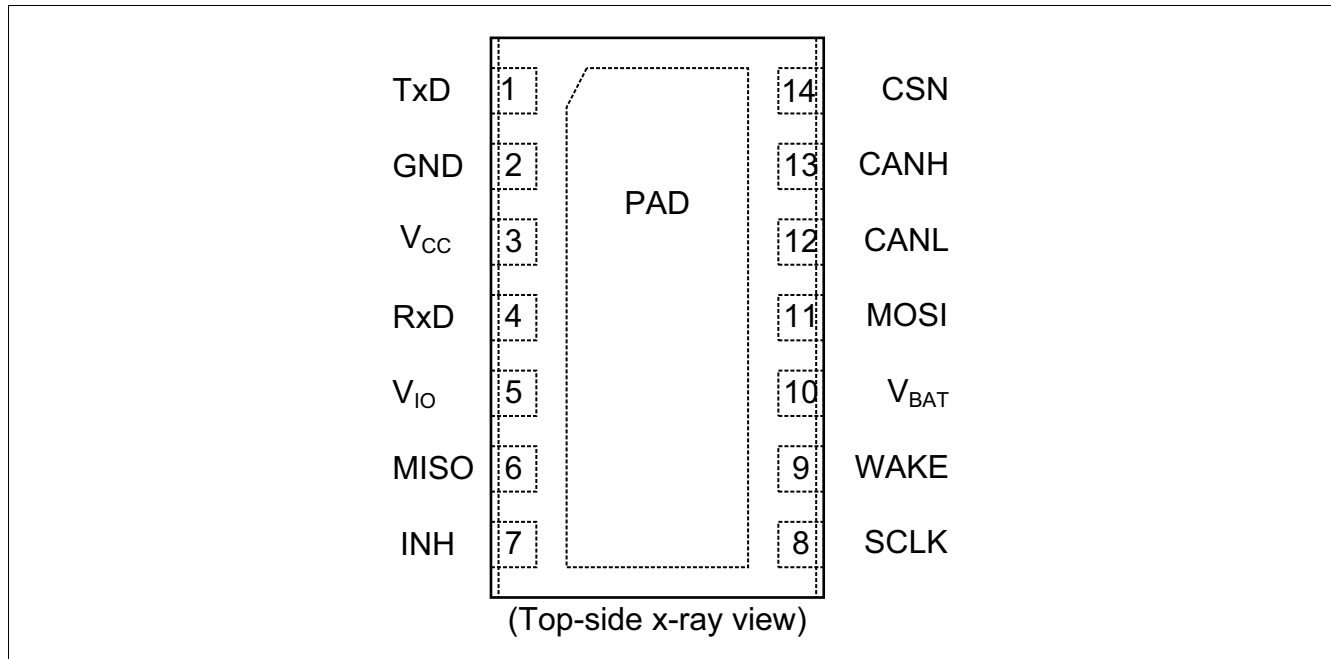
Figure 2 Pin configuration for PG-TSON-14
