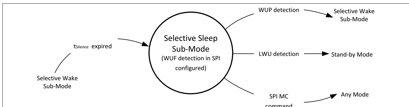
Figure 13 Mode change in Selective Sleep Sub-Mode
