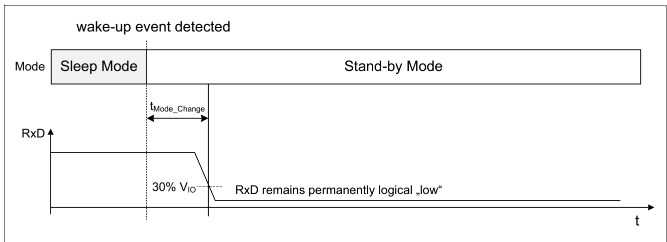
Figure 21 RxD “low” after wake-up event (permanently supplied V_{\text{IO}} )
