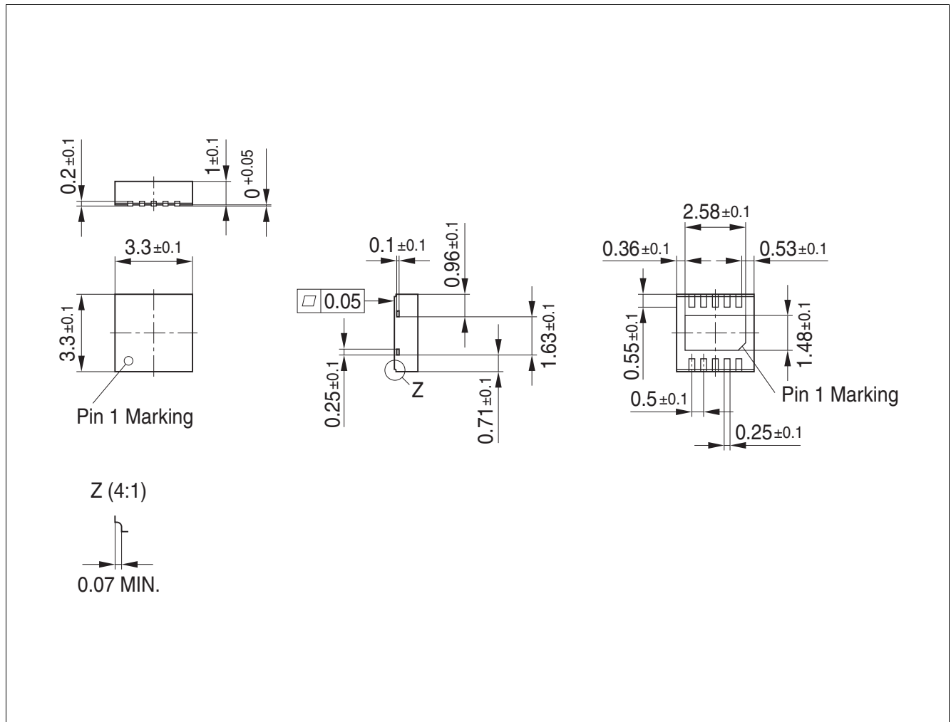
Figure 12 PG-TSON10
