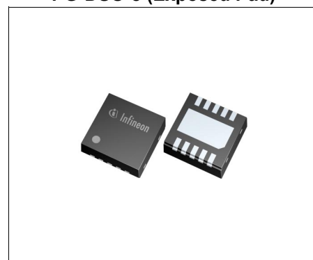
PG-TSON10
