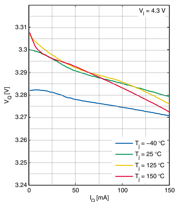
Load Regulation Output Voltage V_Q vs. Load Current I_Q (TLS202B1MBV33)
