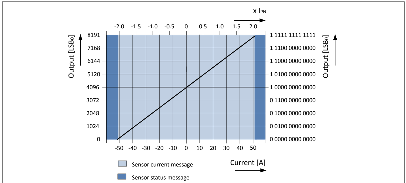
Figure 4 Transfer function
