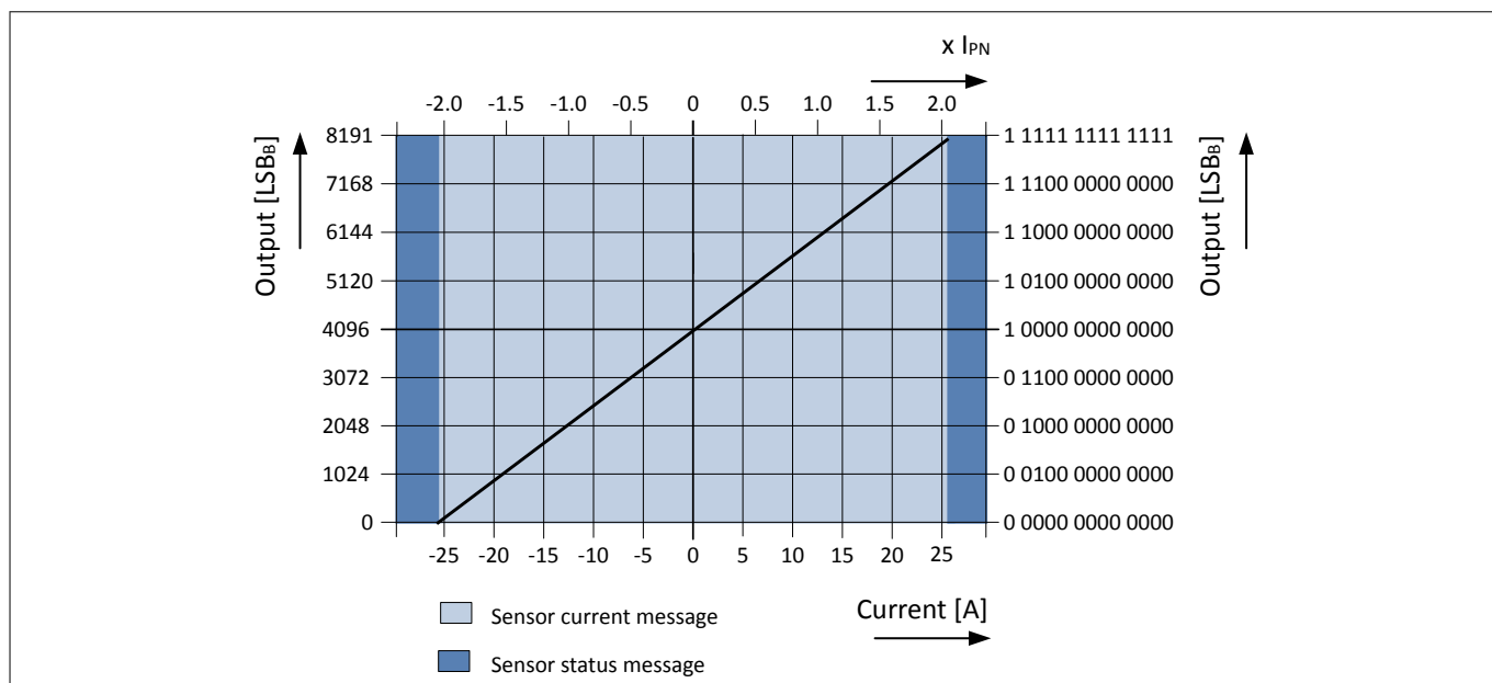
Figure 4 Transfer function
