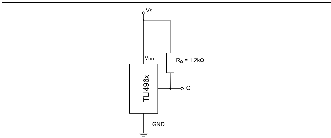
Figure 7 Application circuit
