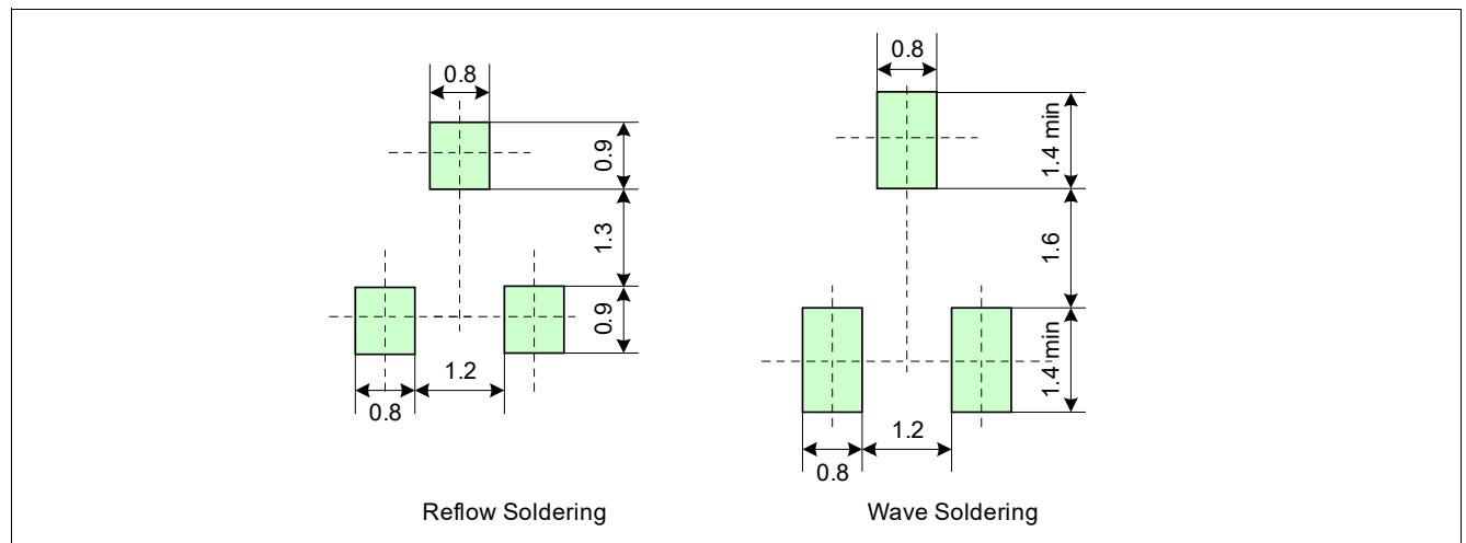
Figure 11 Footprint PG-SOT23-3-15
