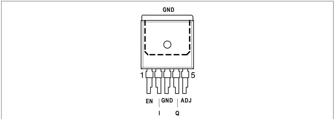
Figure 2 Pin Configuration PG-T0263-5
