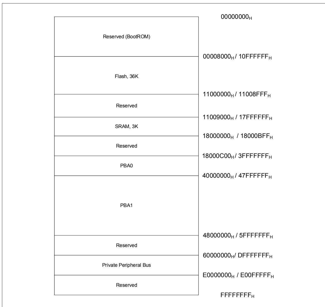
Figure 14 TLE9871QXA20 Memory Map
