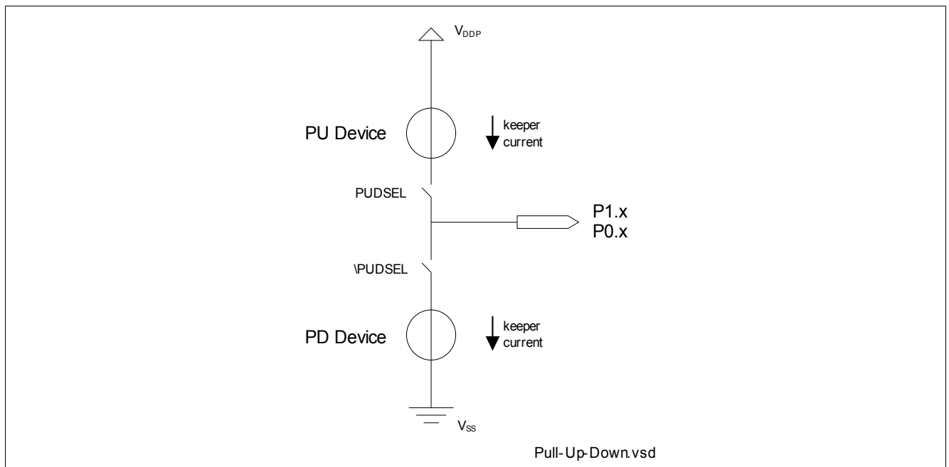
Figure 33 Pull-Up/Down Device
