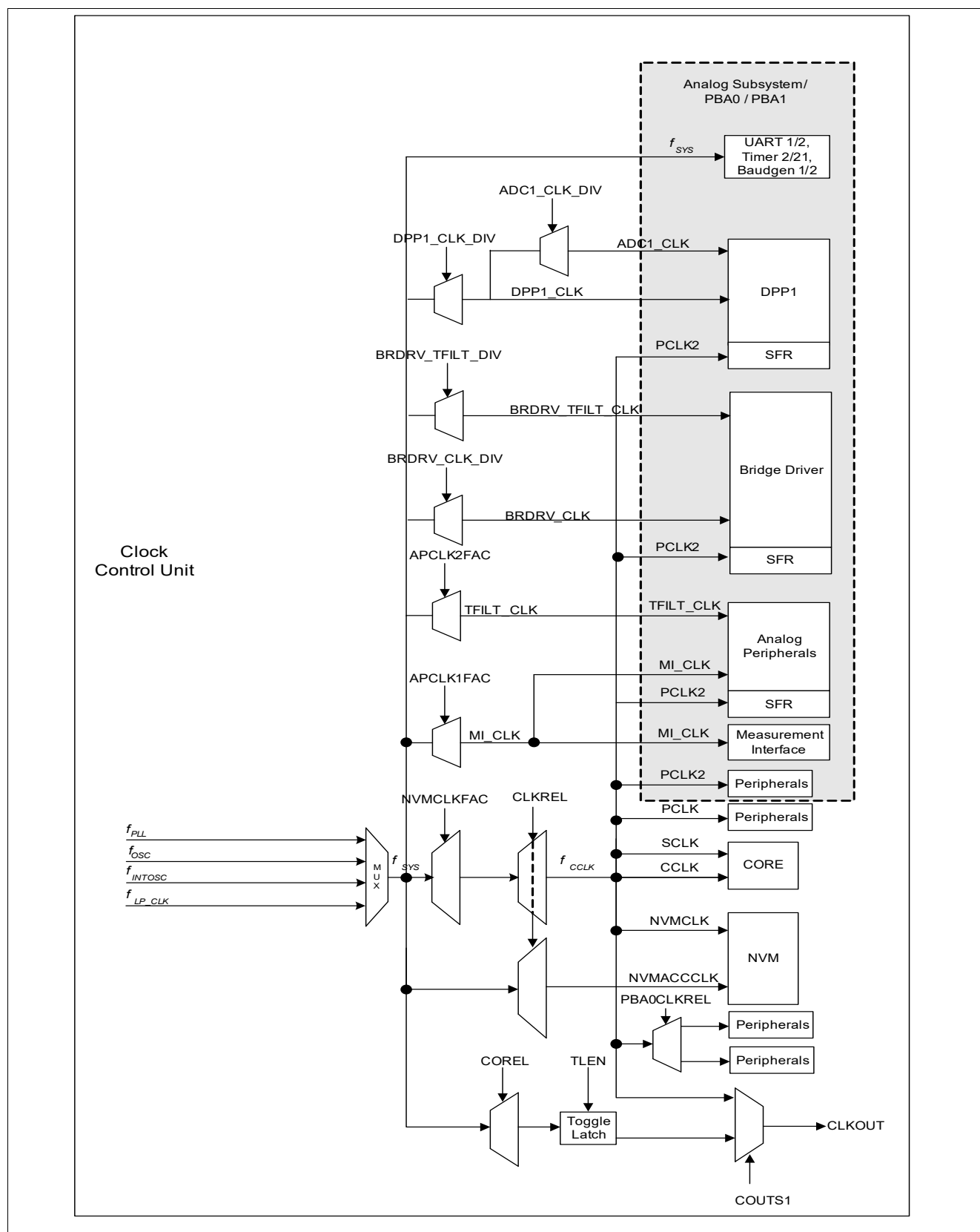
Figure 13 Clock Generation from f_{sys} ; CLKOUT Generation
