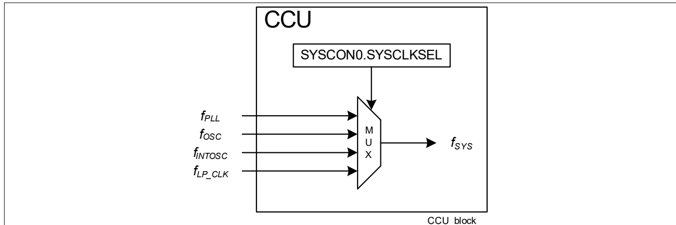
Figure 12 Clock Inputs to Clock Control Unit
