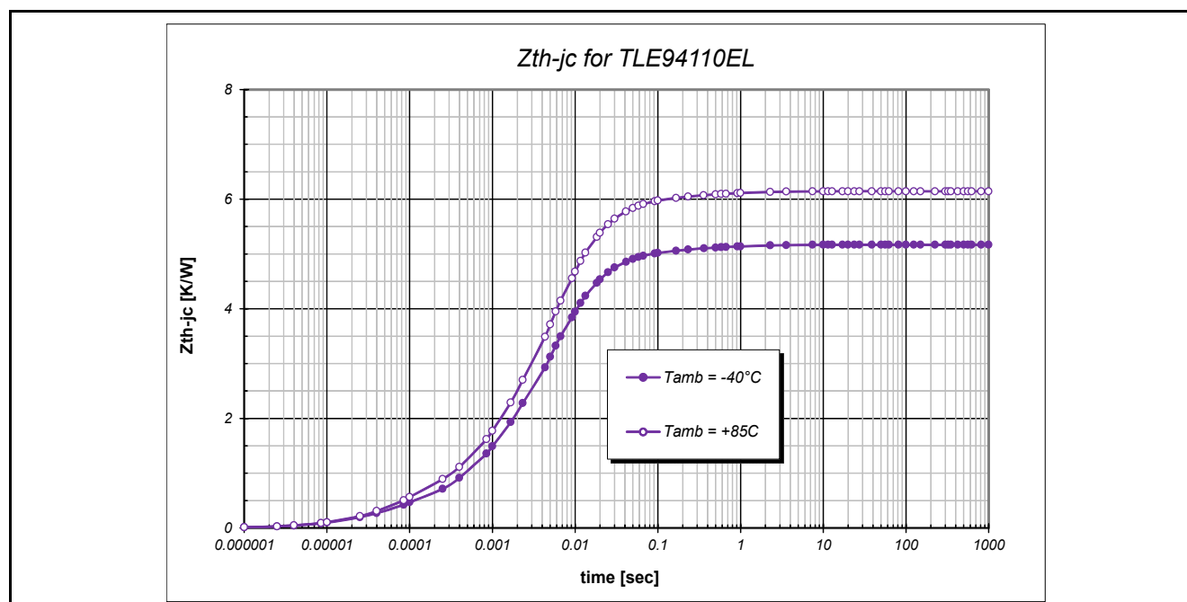
Figure 30 ZthJC Curve
