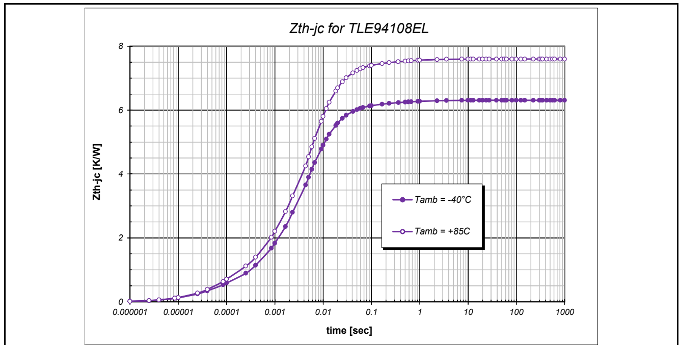
Figure 30 ZthJC Curve
