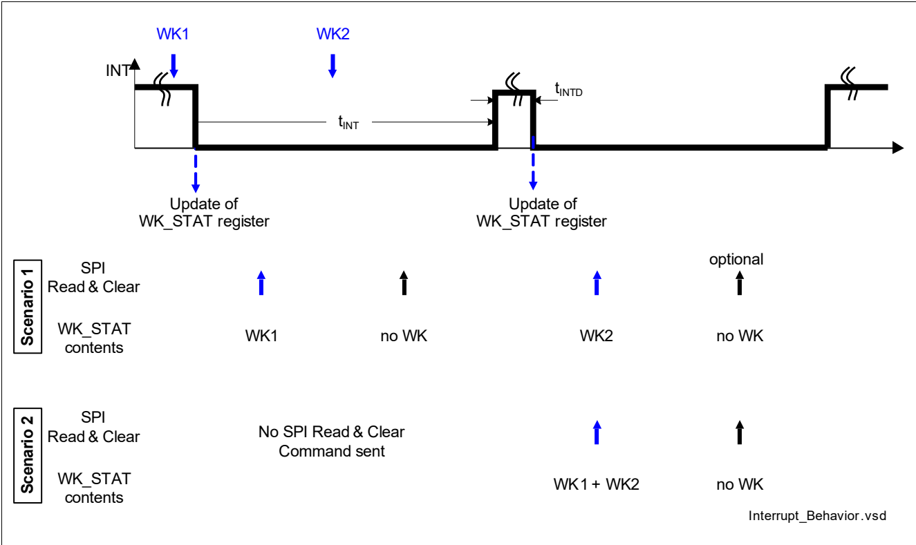
Figure 43 Interrupt Signaling Behavior
