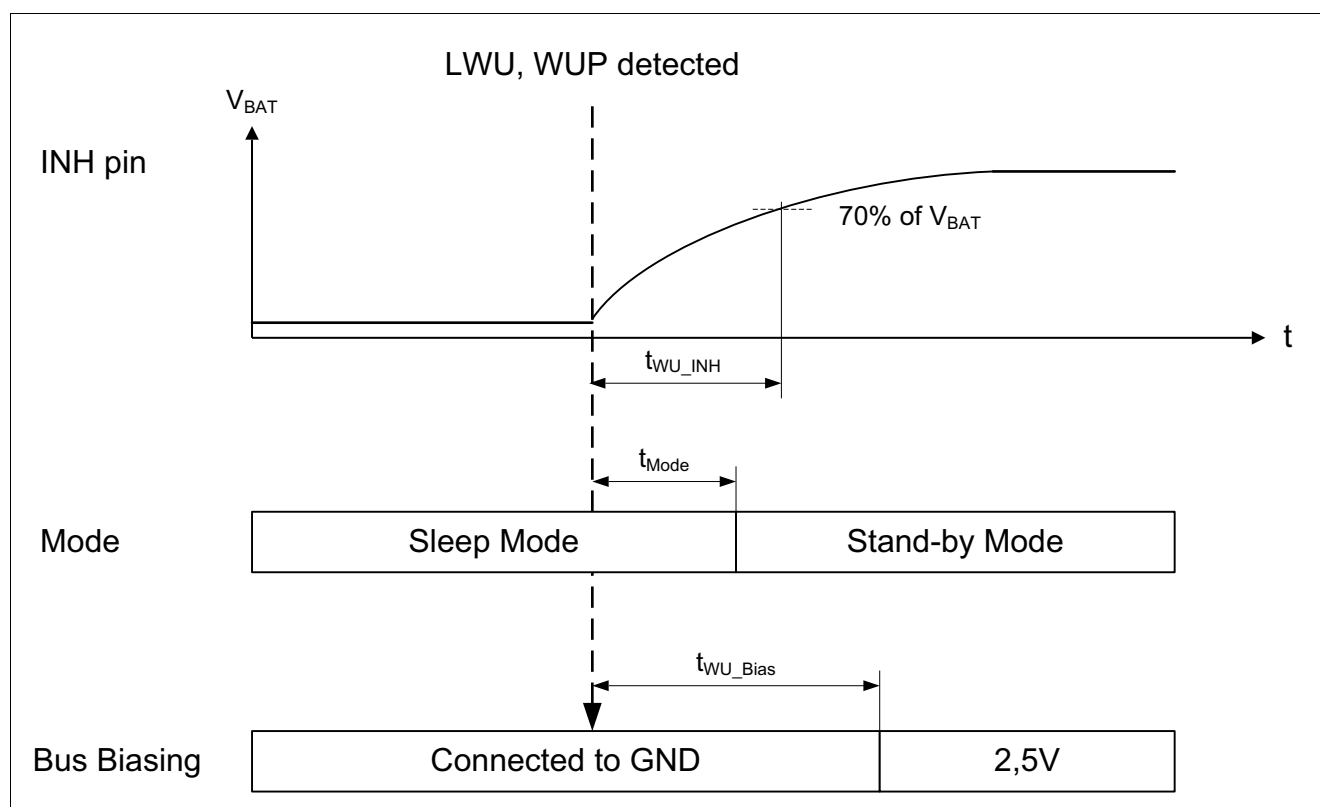
Figure 33 Wake-up detection
