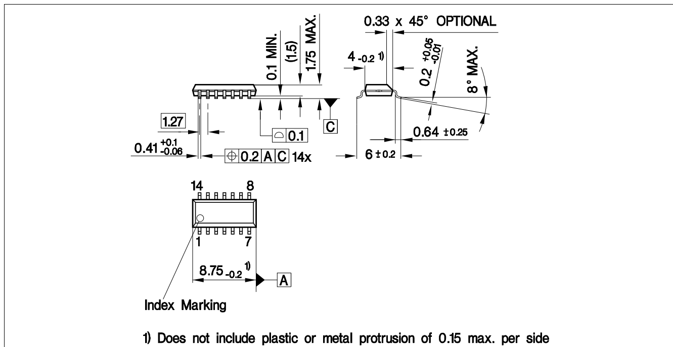
Figure 35 PG-DSO-14
