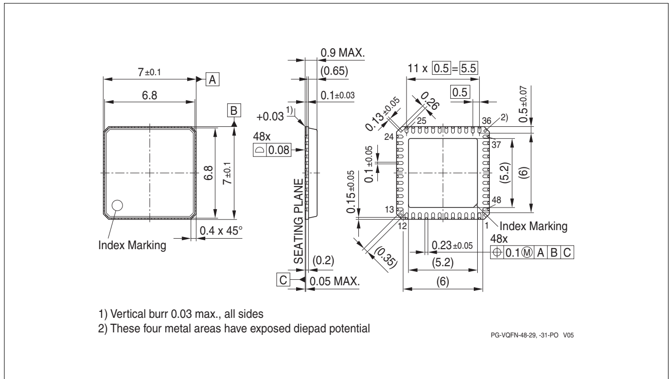
Figure 17 PG-VQFN-48 1)
