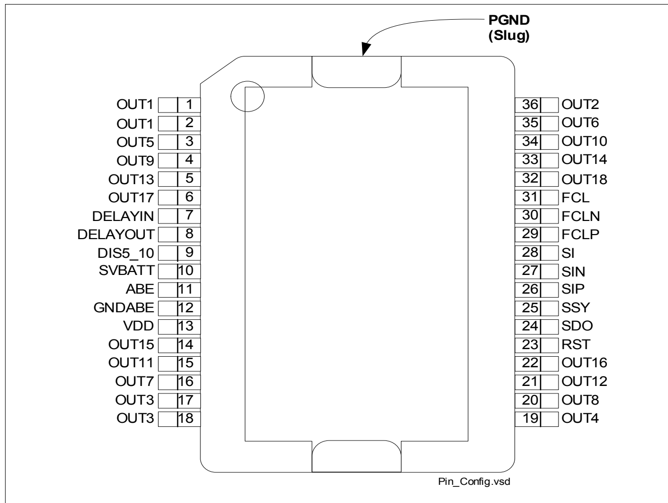
Figure 3 Pin Assignment
