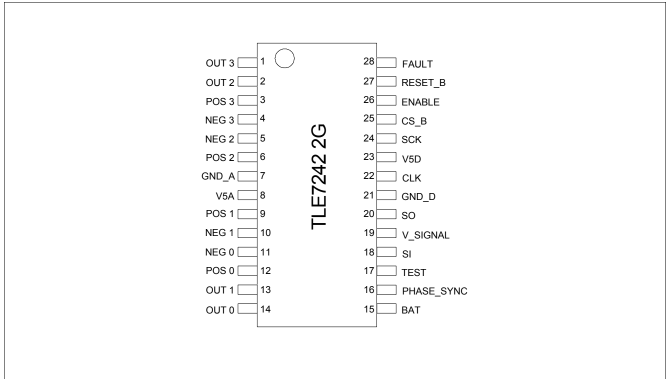
Figure 8 Pin Configuration
