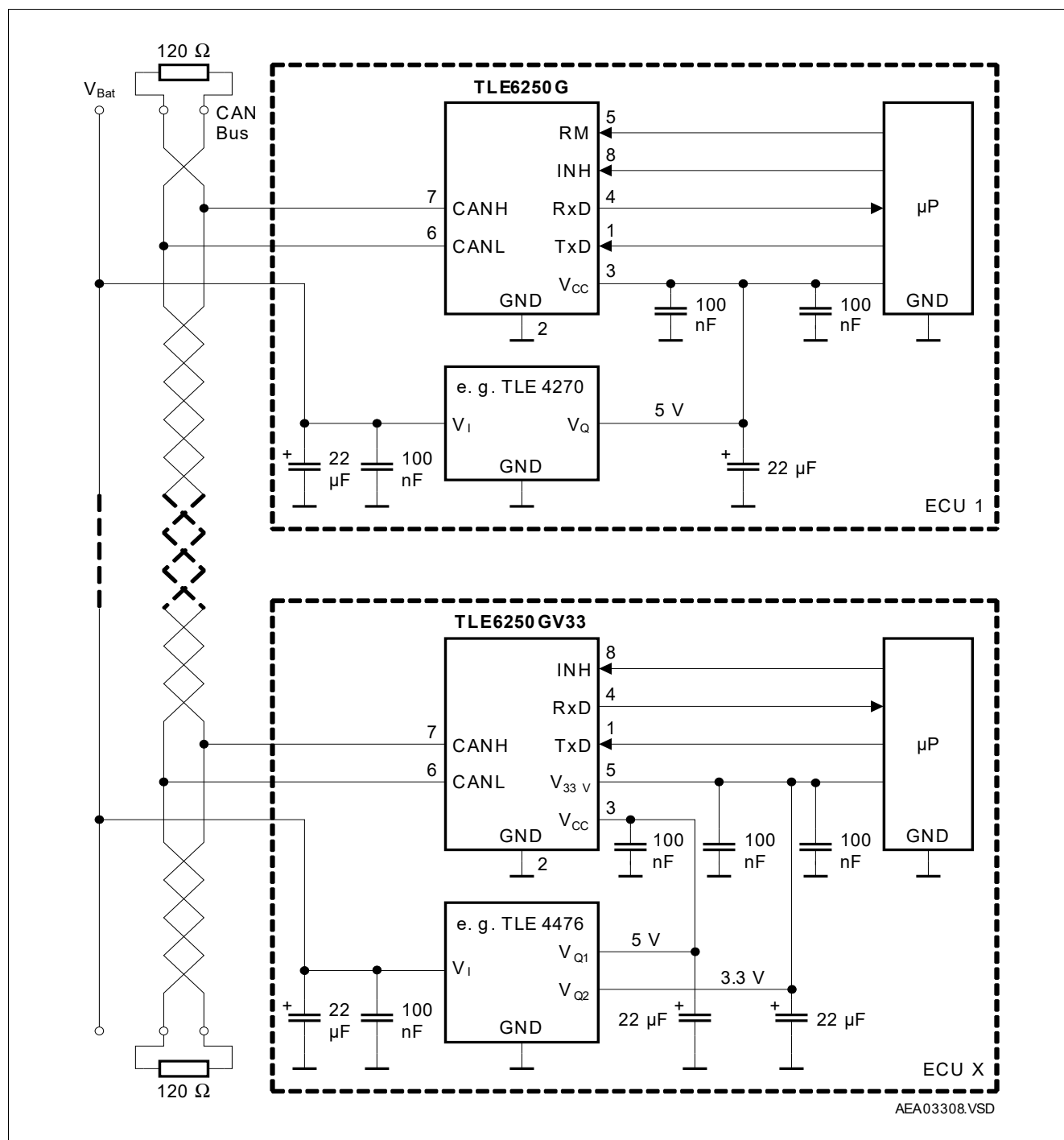
Figure 8 Application circuit TLE6250G with TLE6250GV33
