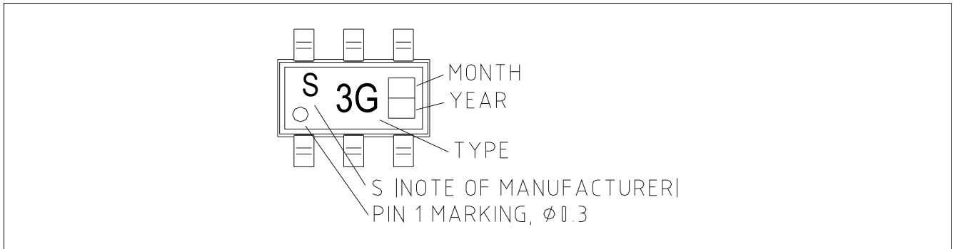
Figure 7 Marking PG-TSOP6-6-9
