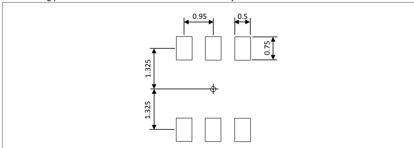
Figure 10 Footprint PG-TSOP6-6-9
