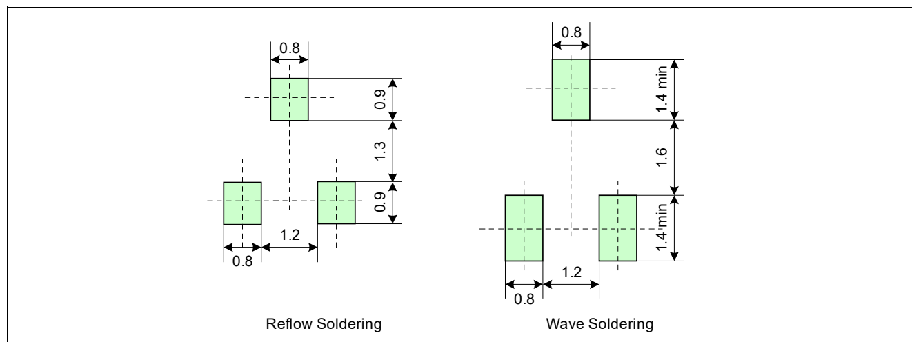
Figure 13 Footprint PG-SOT23-3-15
