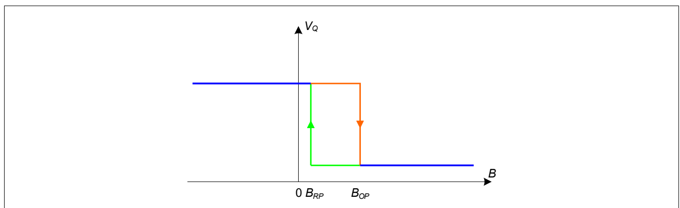
Figure 5 Output signal TLE4964-2K
